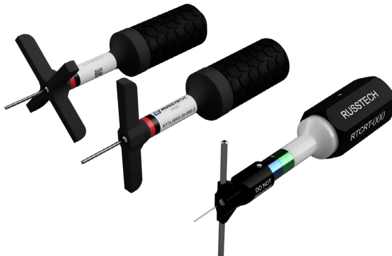
The contact retention tools. From left to right: 3D printed tool with four wings, with two wings, and the legacy tool.
