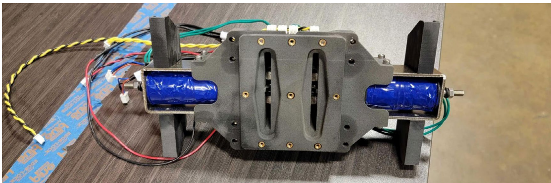
The port of the adapter 3D printed with the Fuse 1 in Nylon 12 Powder.
