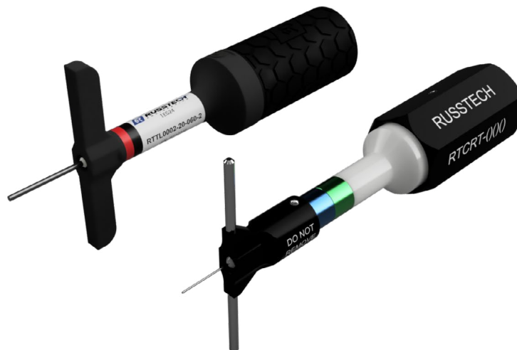
The legacy contact retention tool (right) is an assembly of multiple parts. The body is machined Delrin, the wings are machined stainless steel, and the wing stop safety feature and handle are machined aluminum. The new tool (left) is almost entirely SLS 3D printed in Nylon 12. All versions have a metallic probe at the front.
