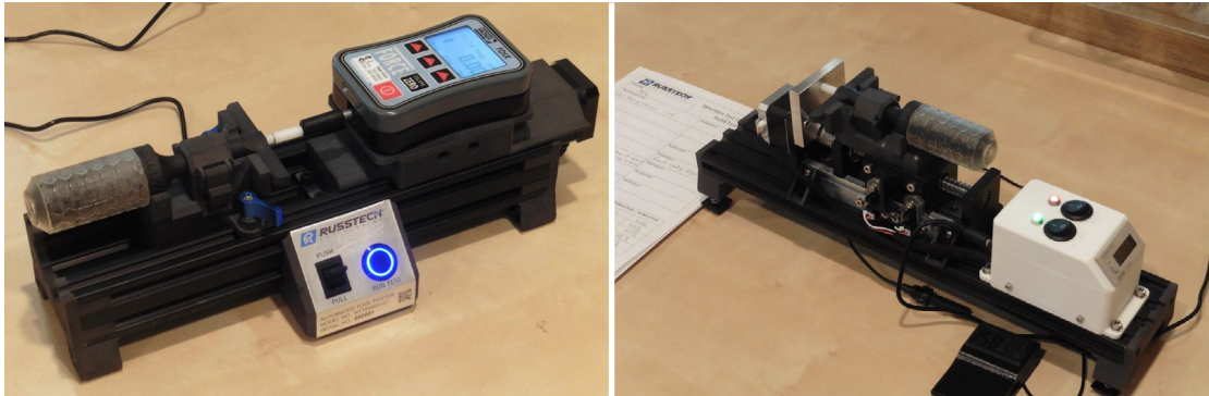
Automated Tool Tester (left) and cycle tester (right). A prototype of the contact retention tool is inserted in the testers. The tool grip is 3D printed in Elastic Resin on the Form 3 printer and will be injection molded in black TPE for the commercialized version, while the core of the tool will remain 3D printed in Nylon 12 with the Fuse 1. The tests are run using a specifically designed Delrin test probe. This specific unit is calibrated to a 6 pound force with a tolerance of \pm 0.5 pound.
